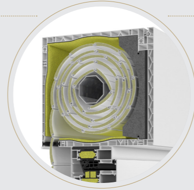
STRUGAL SC LINE ACOUSTIC 185 | 200
